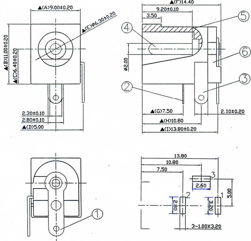
Pin Hole Layout (Jack Bottom View)
